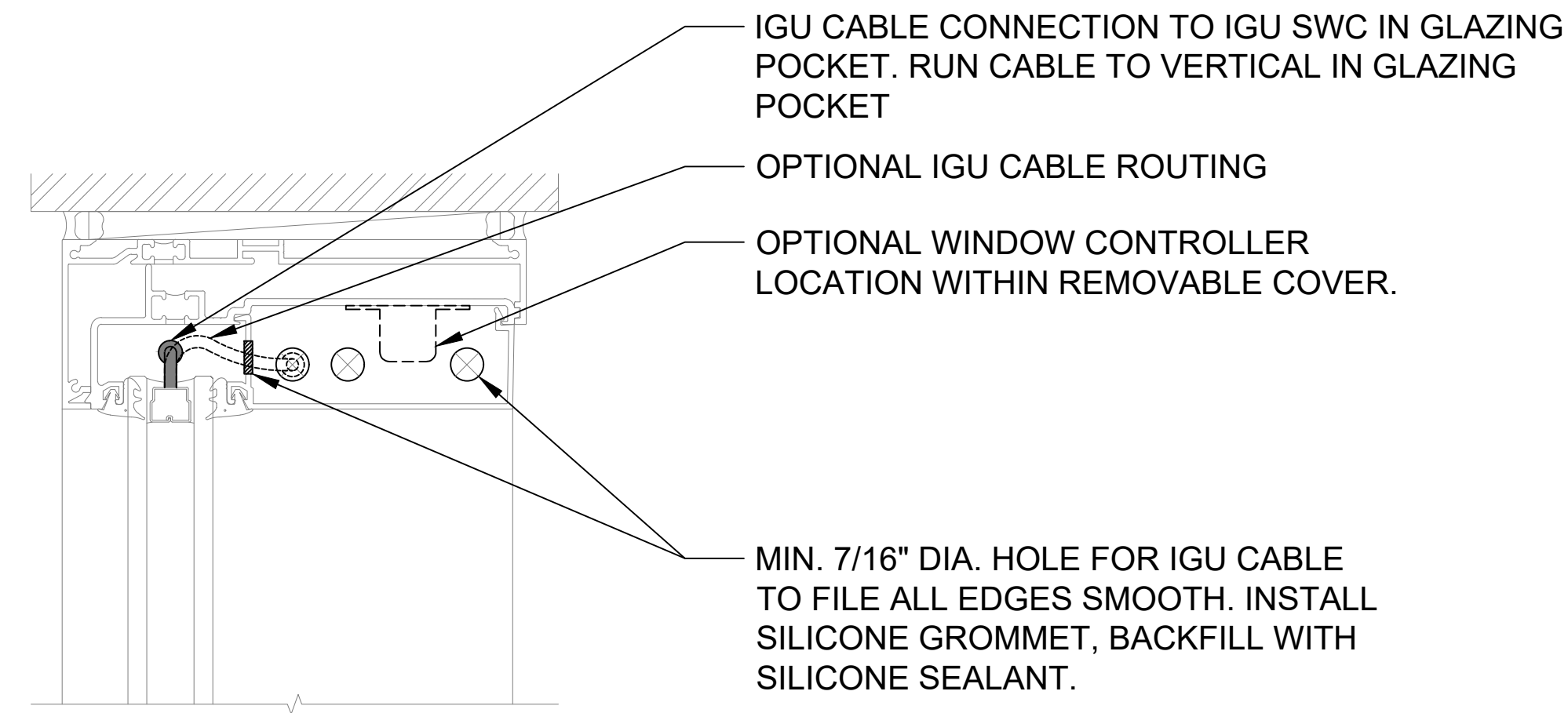
DETAIL 1 HEAD
