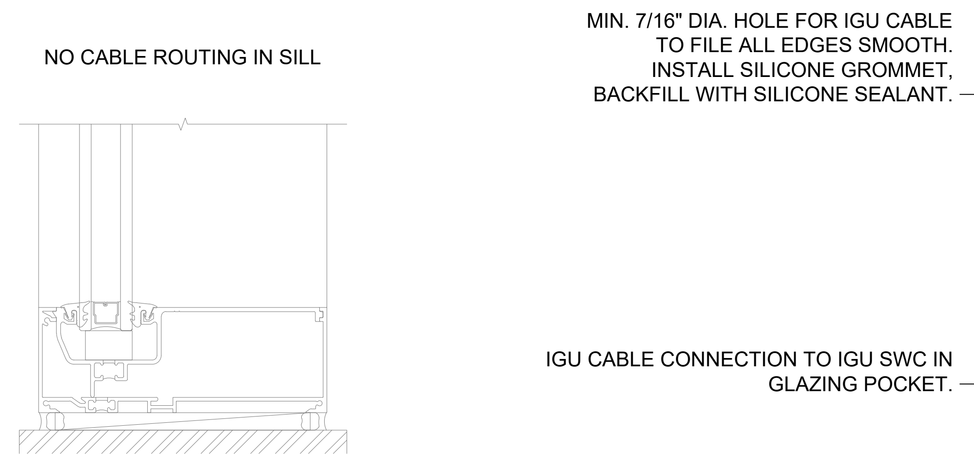
DETAIL 3 SILL
