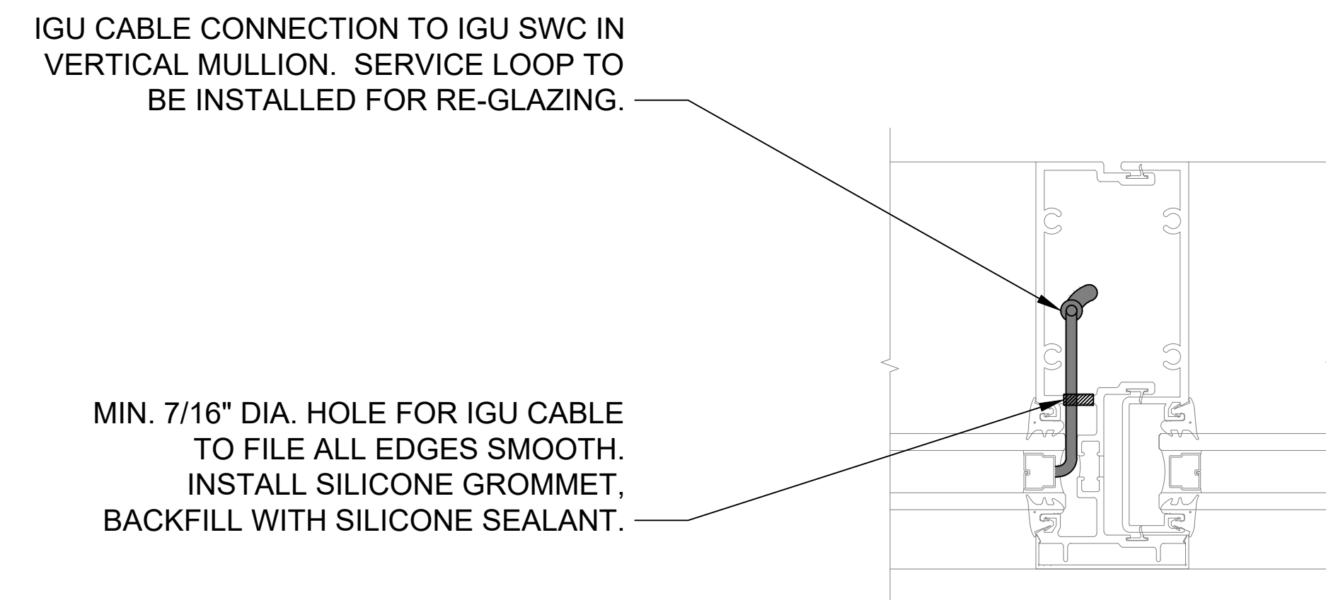
DETAIL 5A VERTICAL EXPANSION MULLION
